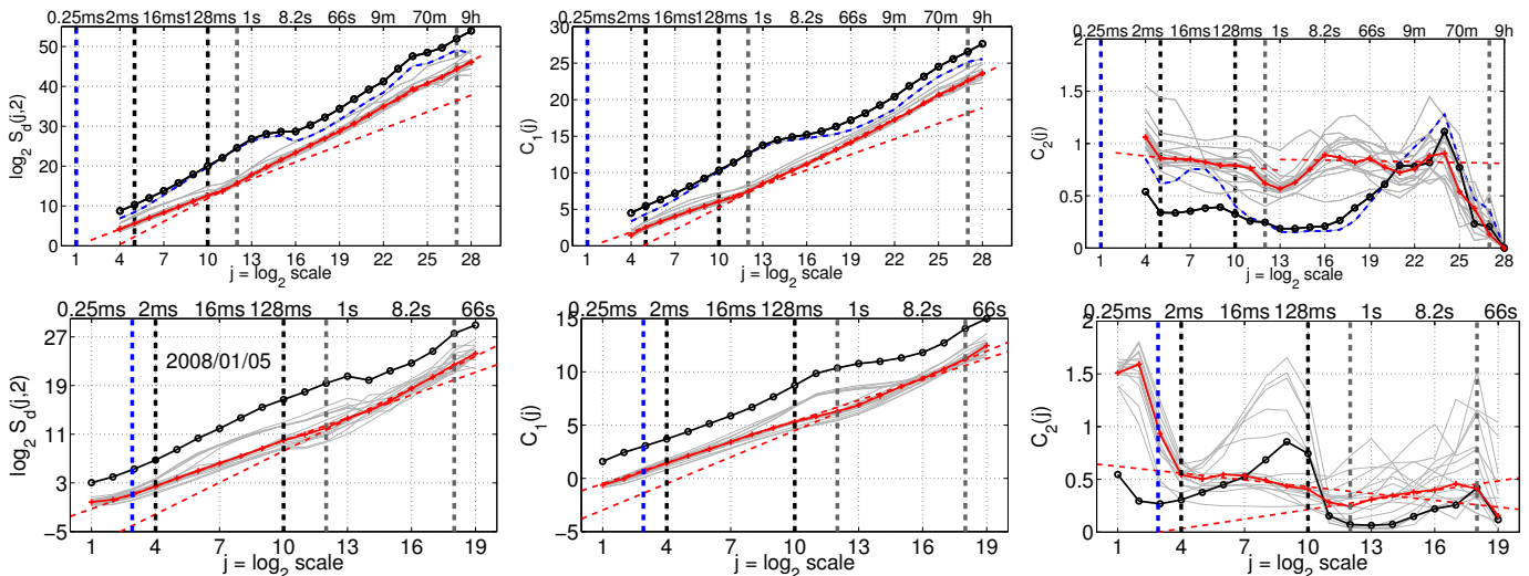
Fig. 2: LDs . From left to right, LDs for the statistics \log_2 S_d(j) , C_1(j) and C_2(j) . Each plot shows Global-LDs (black), Sketch-LDs (light grey), Median-LD (red). Global-LDs are dominated by the Sketch-LD concentrating anomalous traffic (dashed blue). The dashed vertical lines mark respectively the typical IAT time scale j_\tau^M (blue), and the FS (black) and CS (dark grey) scaling ranges ( j_1, j_2 ). Best fits of Median-LDs are shown (dashed-red lines) over both FS and CS. Top: for the 3-day trace. Bottom: for one arbitrarily chosen 15-min trace.
