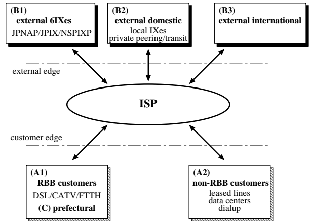
Figure 3: 5 traffic groups at ISP boundary for data collection
