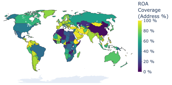
Figure 3: Country-wise ROA Coverage of IPv4 address space in April 2025; Middle Eastern nations have the highest coverage, while China has the lowest among large nations
